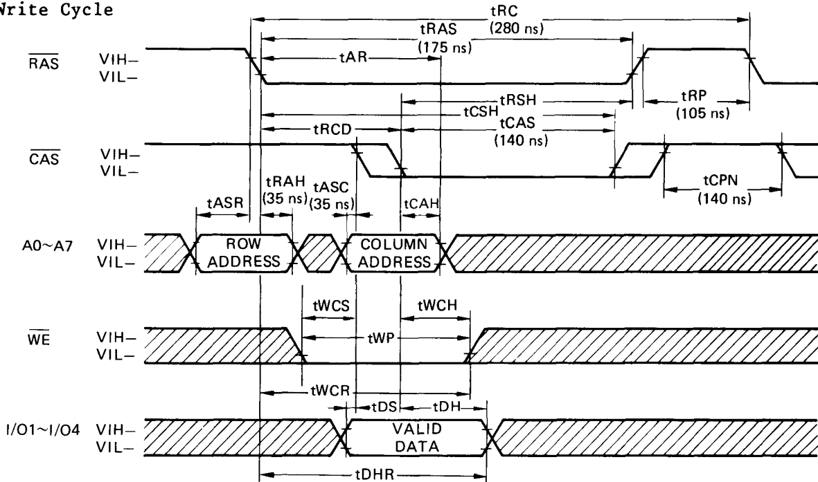
Fig 5-5. DRAM Timing
