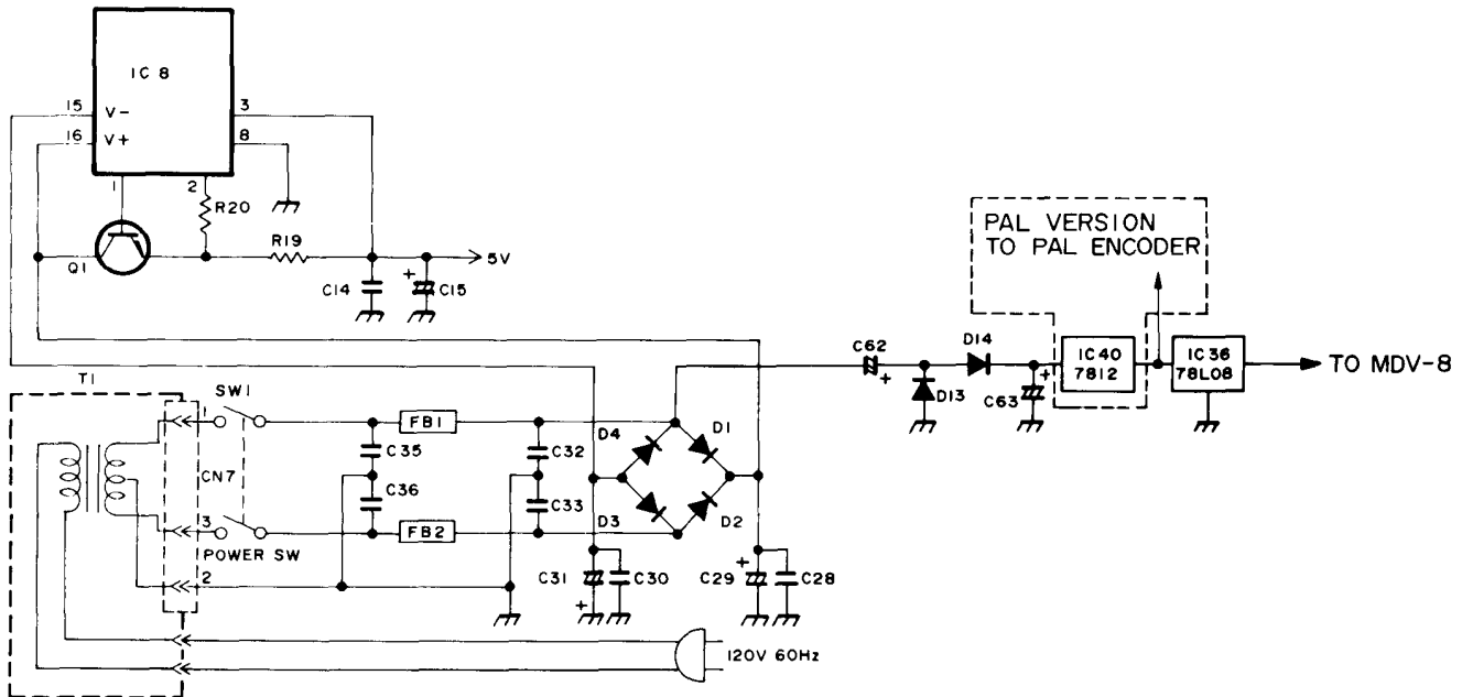
Figure 5-12. Color Computer 3 Power Supply
