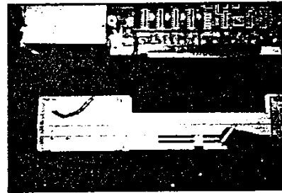
Fig. 3-8. LED Harness Installation
